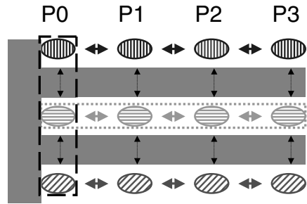
Fig. 10.6. A schematic representation of the CCA parallel programming environment in the single component/multiple data (SCMD) paradigm. Parallel processes, labeled P0, ..., P3, are loaded with the same set of three components. Components in the same process (vertical dashed box) interact using standard CCA port-based mechanisms, while parallel components of the same type (horizontal dotted box) interact using their preferred parallel programming model.
