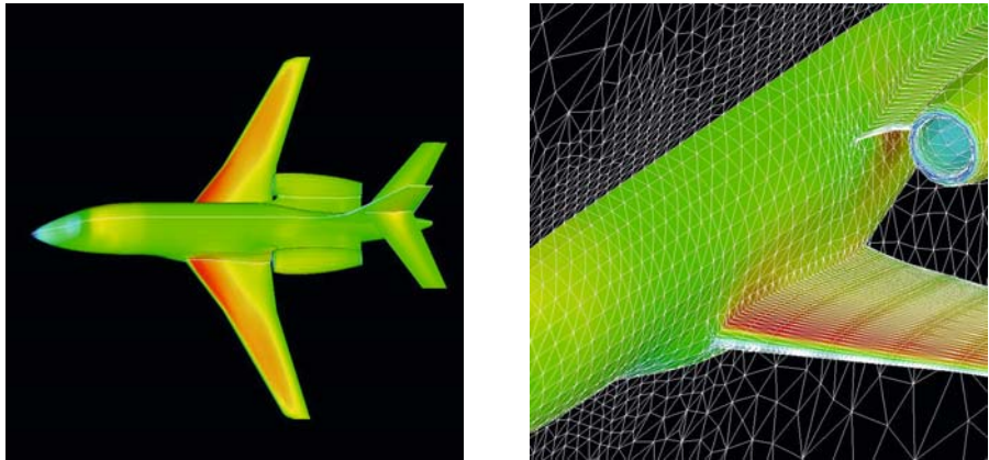
Fig. A.7. Pressure coefficient contours for FALCON_45k. (This is a color version of Figure 4.5 on page 156).
