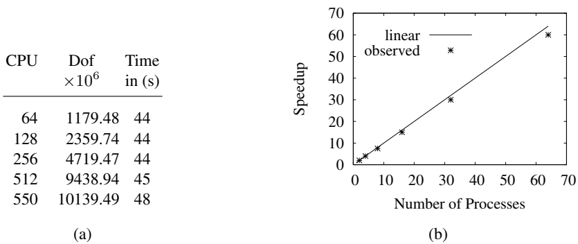
Fig. 5.7. Parallel performance results in 3D: (a) Scalability experiments using a Poisson problem with Dirichlet boundary conditions on an L-shaped domain. Dof denotes the degrees of freedom in the linear system, the timing results given refer to the wall clock time for the solution of the linear system using a full multigrid solver. (b) Speedup results for the same Poisson problem.
