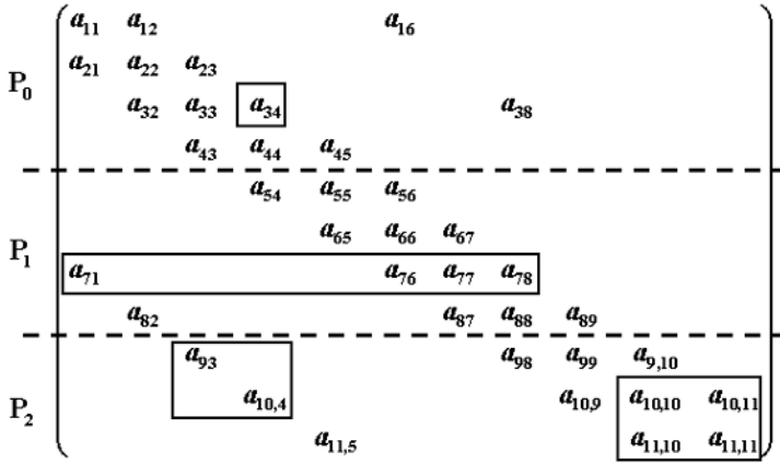
Fig. 8.12. An example of a ParCSR matrix, distributed across 3 processes.
