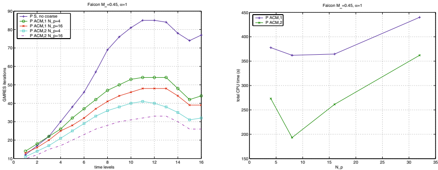
Fig. A.12. FALCON_45k. Comparison among different preconditioners (left) and CPU time, in seconds (right). 16 SGI-Origin3000 processors. (This is a color version of Figure 4.10 on page 159).
