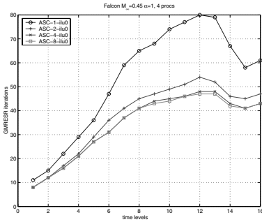
Fig. 4.7. FALCON_45k. Convergence history with 4 (left) and 8 processors (right) with the ASC preconditioner, for different values of L . (For the color version, see Figure A.9 on page 471).
