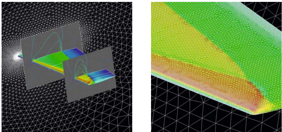
Fig. A.8. Mach number contours for M6_316K. (This is a color version of Figure 4.6 on page 156).
