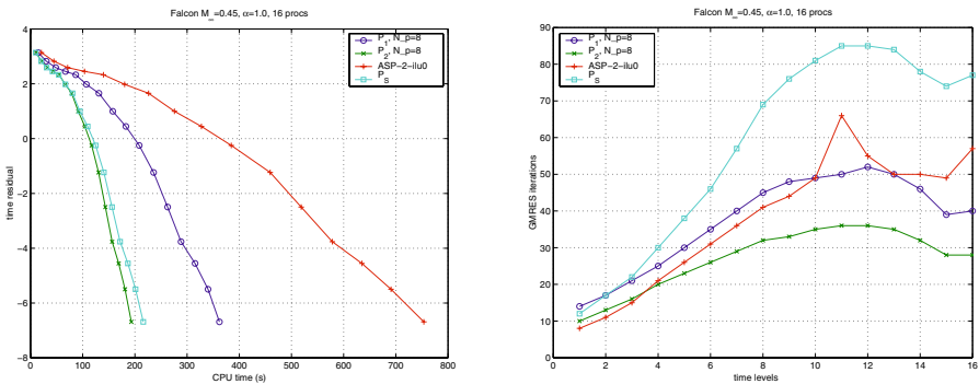
Fig. A.13. FALCON_45k. Residual versus CPU-time (left) and iterations to converge at each time level (right), using 16 SGI-Origin3000 processors. (This is a color version of Figure 4.11 on page 159).
