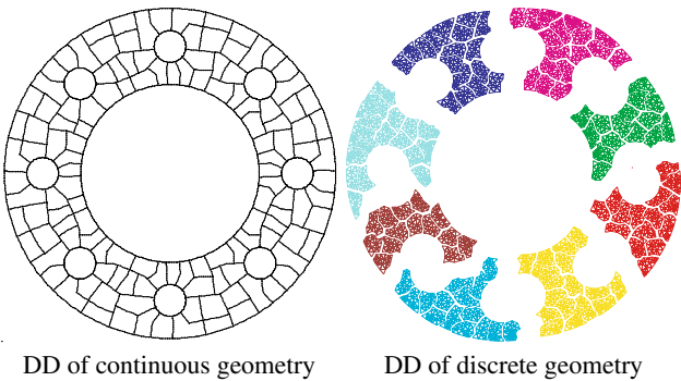
Fig. A.17. Domain decomposition of the continuous geometry [52] and the discrete geometry [17] of a cross section of a rocket pipe. (This is a color version of Figure 7.1 on page 239).
