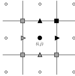
Fig. 8.4. Grid variables in hypr e are referenced by the abstract cell-centered index to the left and down in 2D (and analogously in 3D). So, in the figure, index (i, j) is used to reference the variables in black. The variables in grey, although contained in the pictured cell, are not referenced by the (i, j) index.
