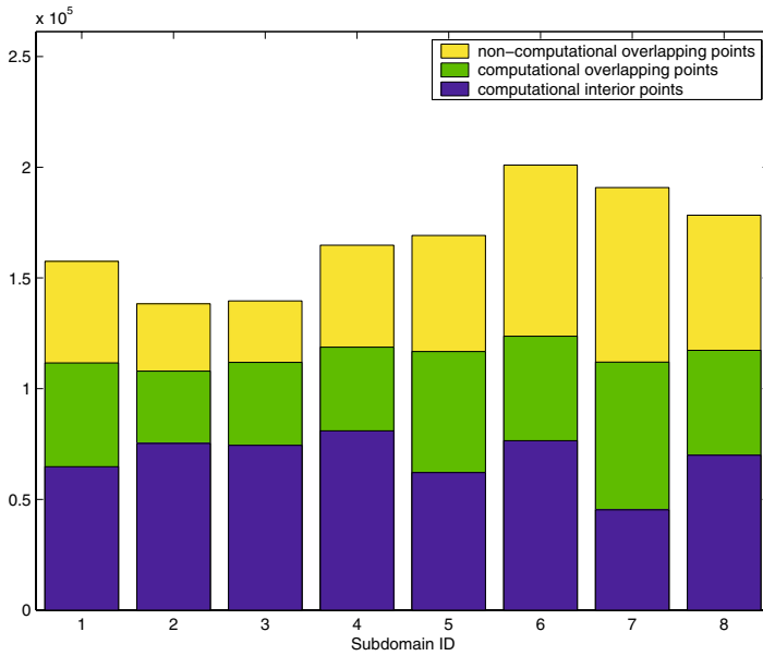
Fig. A.26. The effect of applying a disjoint re-distribution to the \Omega mesh points, where N_{\Omega} = 919, 851 and the number of subdomains is 8. (This is a color version of Figure 11.7 on page 406).
