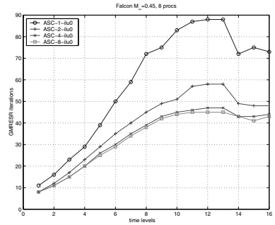
Fig. 4.7. FALCON_45k. Convergence history with 4 (left) and 8 processors (right) with the ASC preconditioner, for different values of L . (For the color version, see Figure A.9 on page 471).
