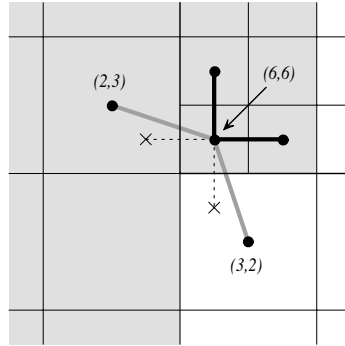
Fig. 8.11. Coupling for equation at corner of refinement patch. Black lines (solid and broken) are stencil couplings. Gray line are non-stencil couplings.
